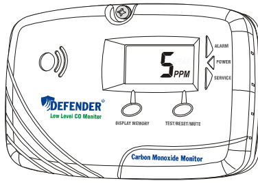
Auto. Displays 5 - 500 PPM (e.g. 5 PPM detected)
